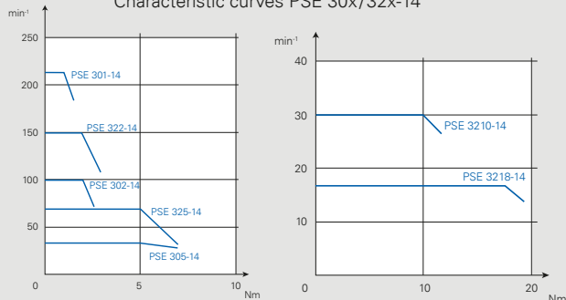
Characteristic curves PSE 30x/32x-14
